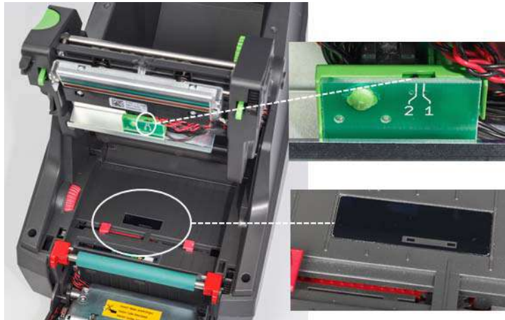
Gap Sensor Detail
